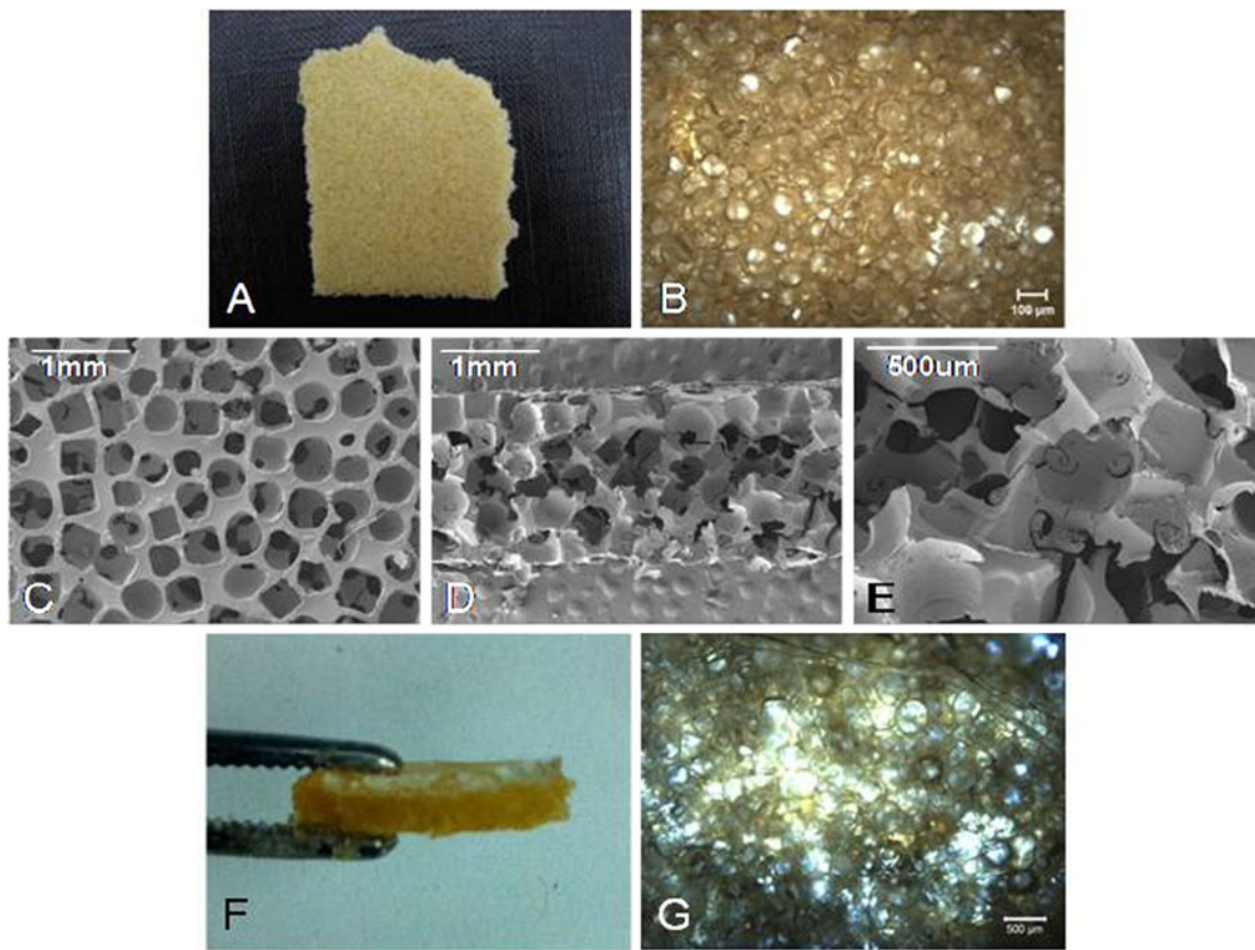
Fig. 2 (A) Image of a 75 wt% EH scaffold. (B) 2.5 \times magnification of a 75 wt% EH scaffold. (C) SEM image of the surface of a 75 wt% EH scaffold. (D) SEM image of the cross-section of a 75 wt% EH scaffold. (E) Higher magnification SEM image of a single pore in a 75 wt% EH scaffold. (F) Image of 80% EH-PEG scaffold. (G) 2.5 \times magnification of 80% EH-PEG scaffold.
